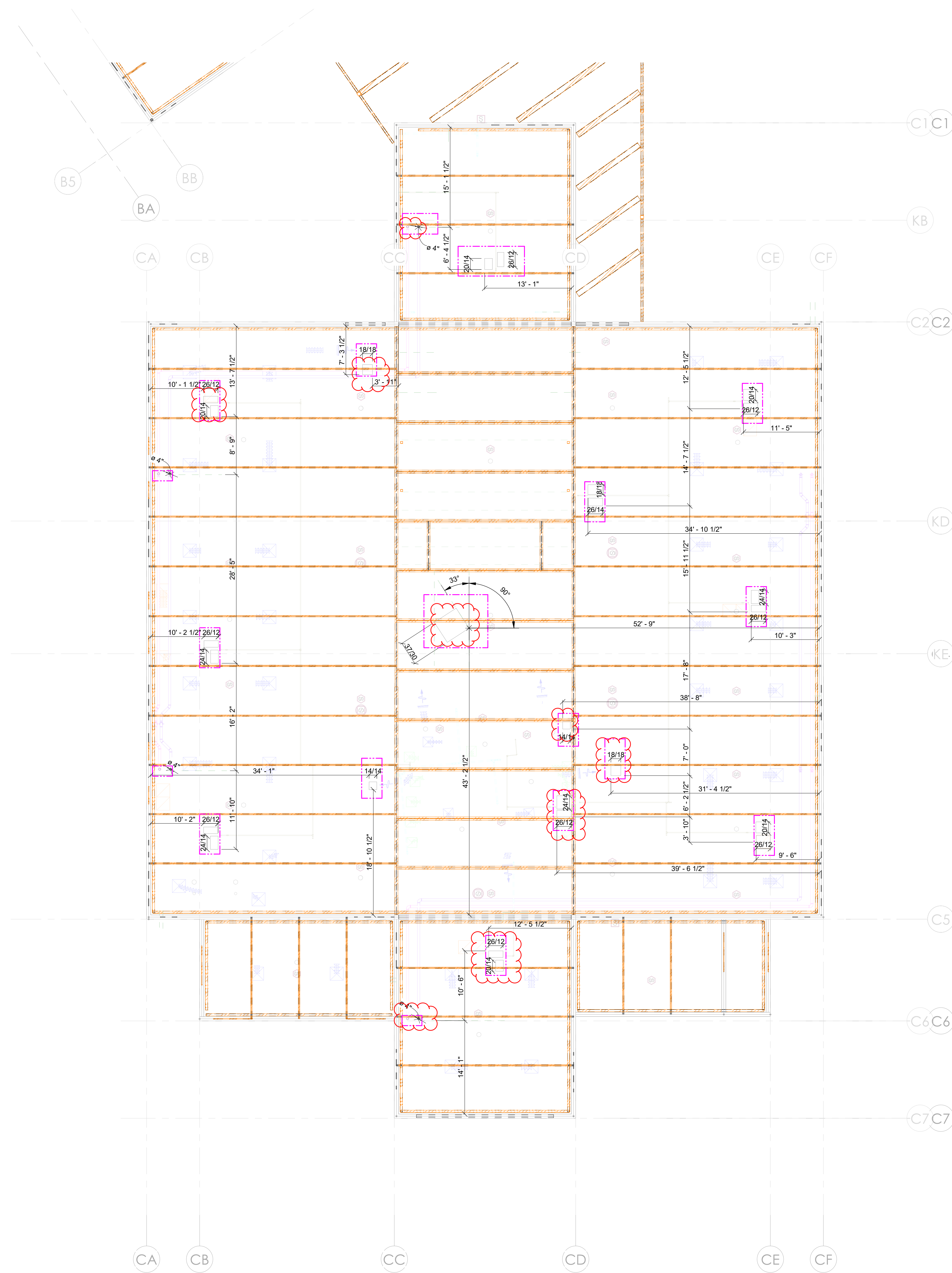
NORTH ↑ (Building C) Penetration Plan - Roof Building K-2 1/8" = 1'-0"
