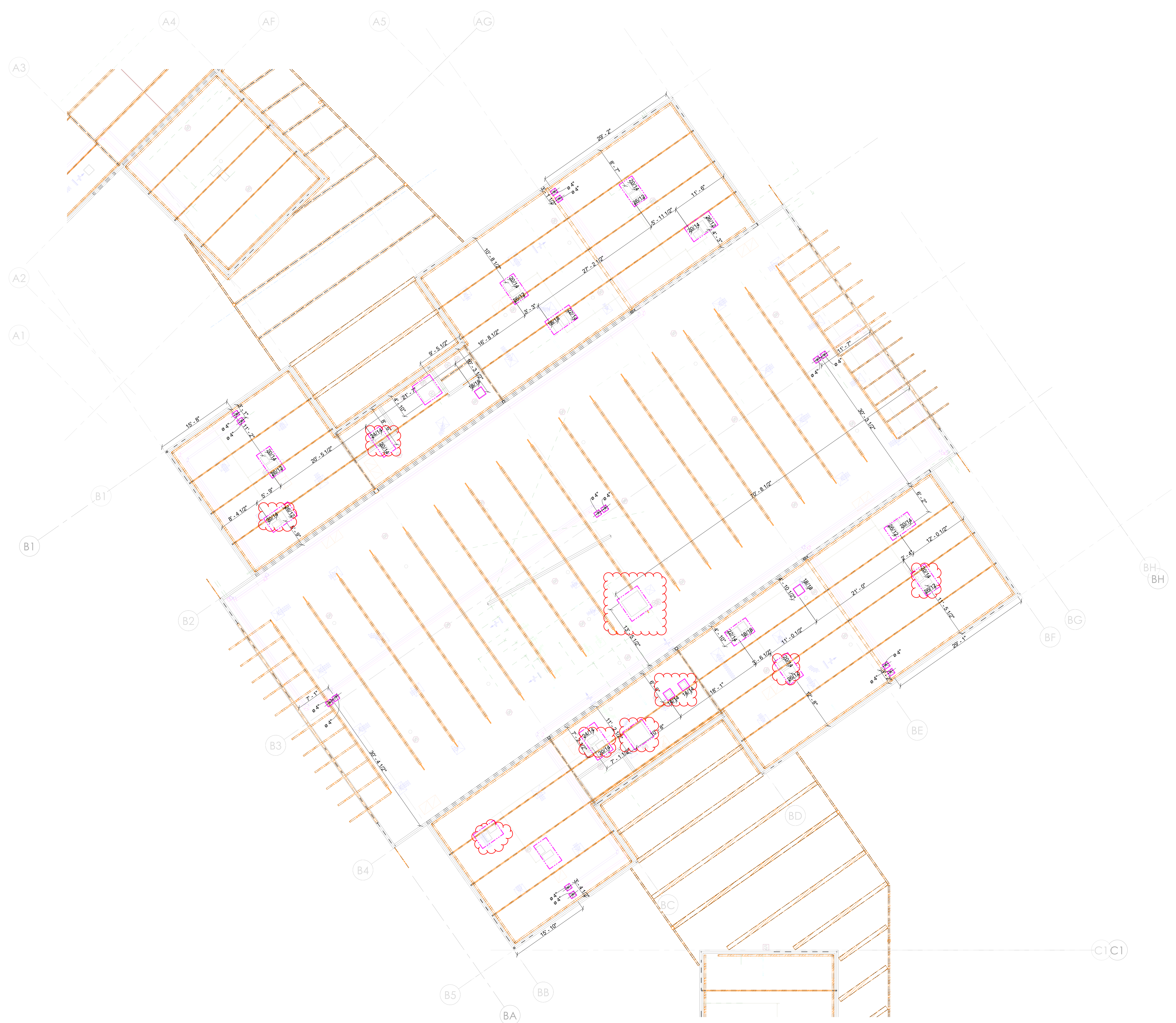
NORTH (Building B) Penetration Plan - Roof Building 6-8 1/8" = 1'-0"
