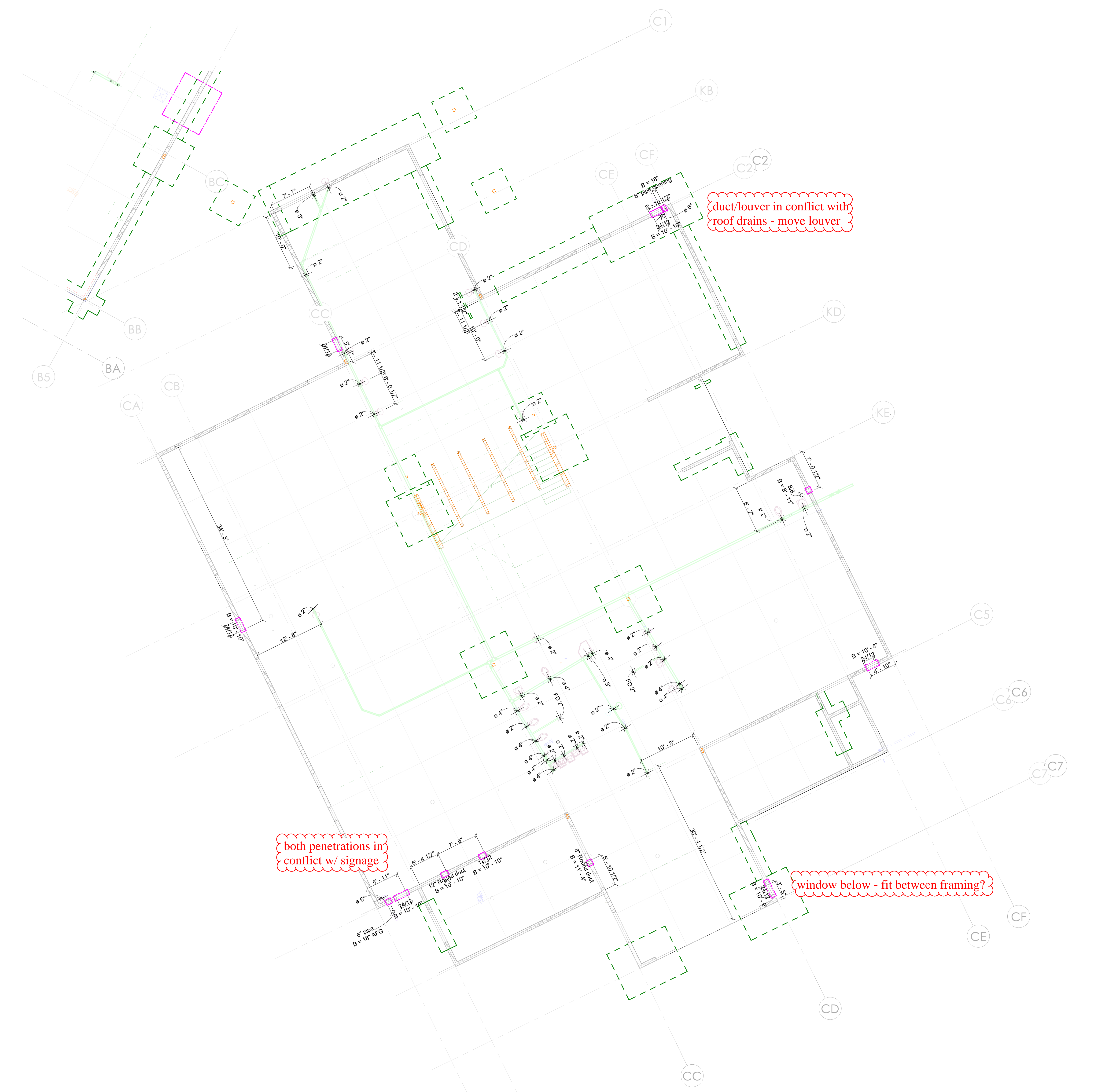
(Building C) Penetration Plan - 1st Floor Building K-2 1/8" = 1'-0"
